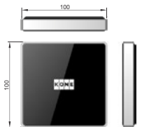
KDS Home, Landing Call Station
